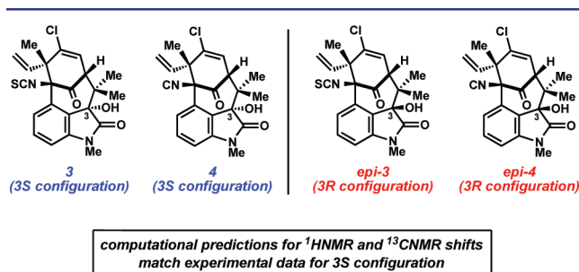
Figure 4. Structures of 3 and 4 , in addition to C3 epimers, and summary of computational findings.
